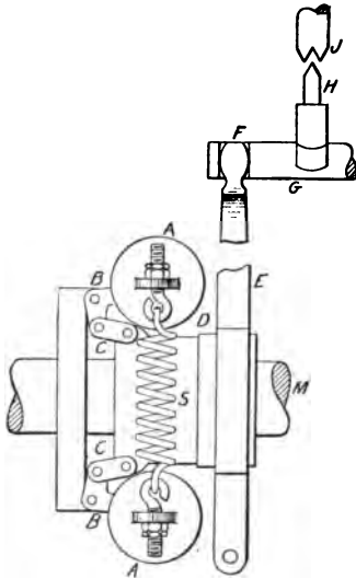
FIG. 213.—One type of Gas Engine Governor, which is an improved variation of the device used on the early Daimler motors. The parts are as follows: A and A, ball weights; B and B, bell cranks actuating the links. C and C, as the balls move outward resisting the tension of spring, S, and sliding sleeve, D, on the shaft, M. E is a lever arm attached to D, which moves the shaft, G, by contact at F, as shown, thus throwing the pick blade, H, out of contact with the end, J, of the exhaust valve rod.
